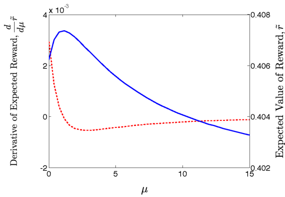
Fig. 3. The derivative of the expected value of reward for the matching shoulders reward structure shown in Figure 1. The dotted line is \frac{d}{d\mu}\tilde{r} from Equation (28). The solid line is the expected value of reward, \tilde{r} . Both are plotted against \mu for N = 20 .
