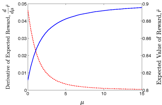
Fig. 4. The derivative of the expected value of reward for the converging gaussians reward structure shown in Figure 2. The dotted line is \frac{d}{d\mu}\tilde{r} from Equation (28). The solid line is the expected value of reward, \tilde{r} . Both are plotted against \mu for N = 20 .
