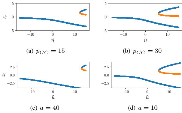
Fig. 1. Bifurcation diagram of (16) in the prisoner's dilemma with (a) p_{CC} = 15 and (b) p_{CC} = 30 , where \alpha = 0 , d = \gamma = \eta = 1 , p_{CD} = 0 , p_{DC} = 40 , p_{DD} = 5 , and in the public goods game with (c) a = 40 and (d) a = 10 , where \alpha = 0 , d = \gamma = \eta = 1 , \rho = 2 , and N_a = 20 . Blue (orange) curves are stable (unstable) equilibrium states. Solutions with z_c < 0 ( z_c > 0 ) correspond to mutual defection (cooperation). Mutual defection is always stable; for large enough \tilde{u} , mutual cooperation is stable.
